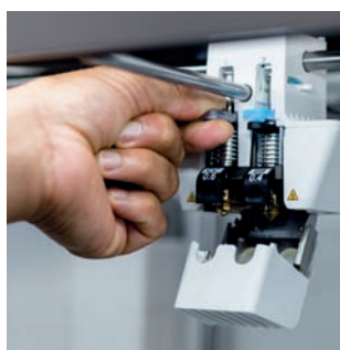
Print core CC 0.6 mm Ruby-tipped for printing abrasive composites
